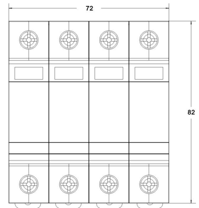
Outline dimension
