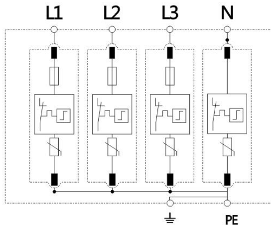
Electrical principle
